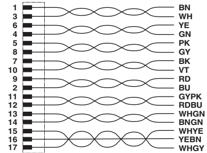
Contact assignment of the M12 plug
